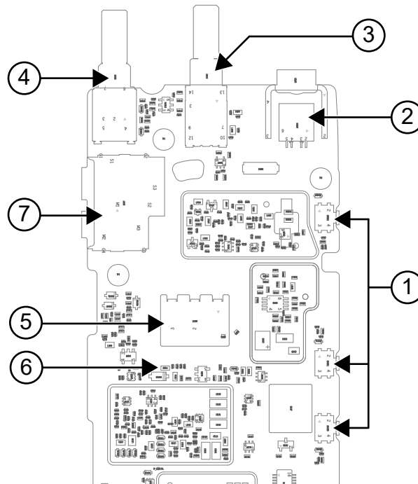
Figure 5: Main Board Top Side for UHF1, UHF2, and 350 MHz Band
